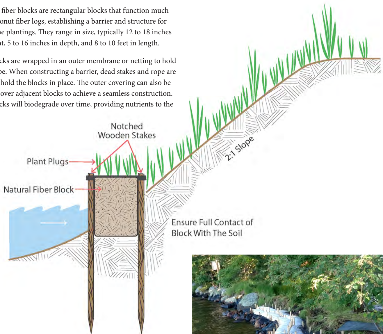
FIGURE 4: NATURAL FIBER BLOCK
