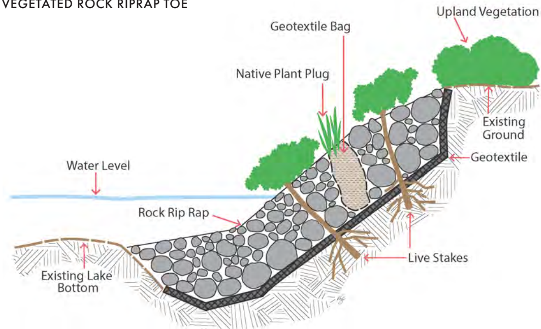
FIGURE 10: VEGETATED ROCK RIPRAP TOE
