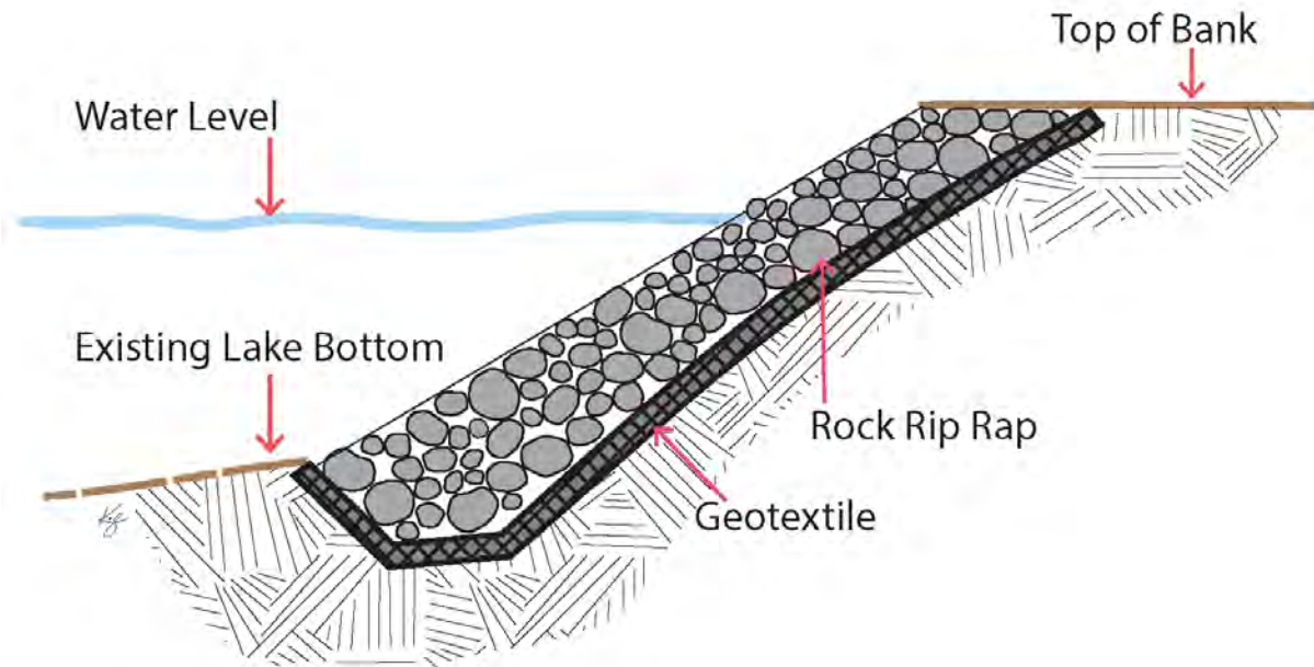
FIGURE 8: ROCK RIPRAP TOE WHERE NATIVE VEGETATION CANNOT BE ESTABLISHED
